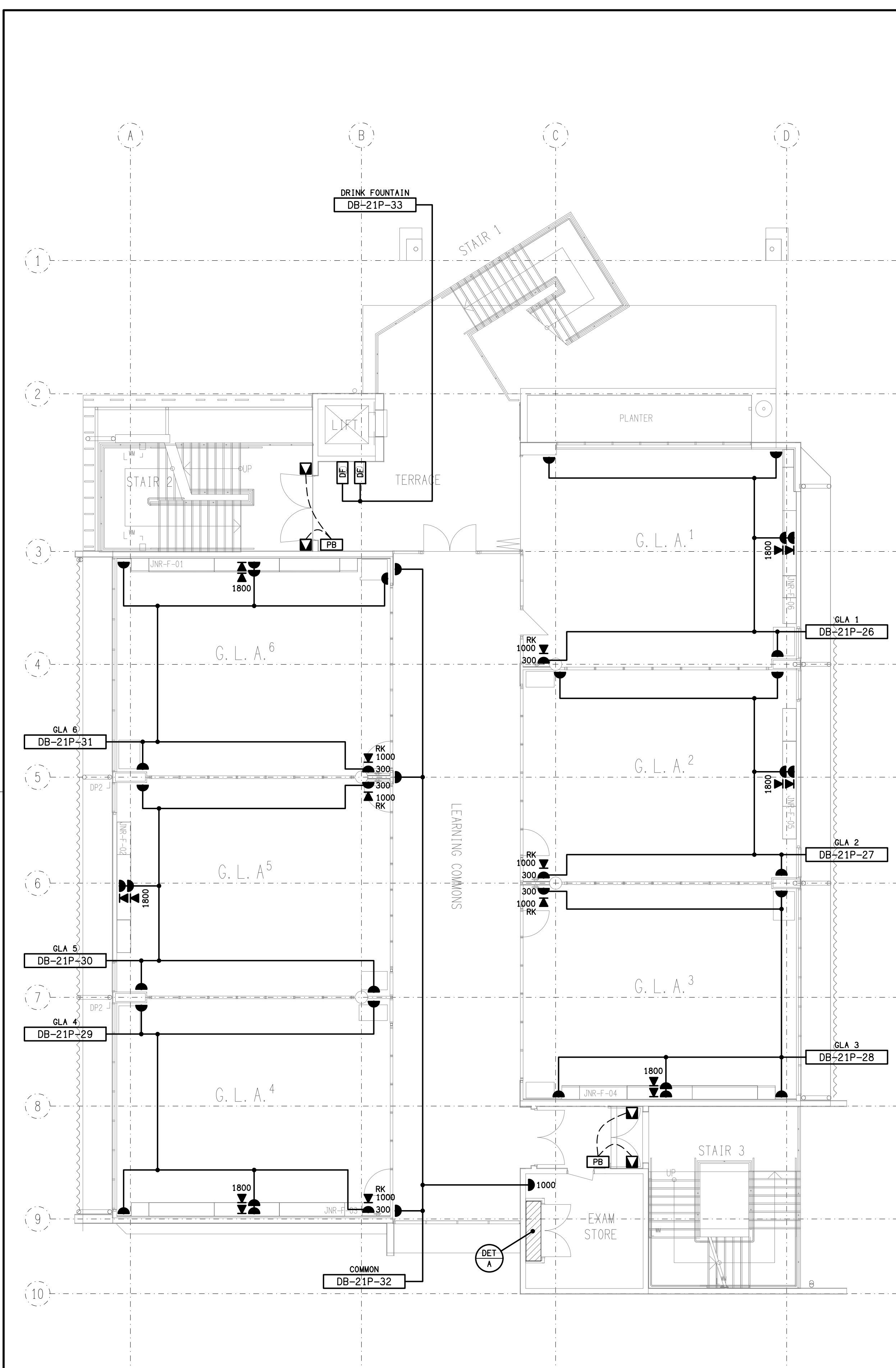
FLOOR PLAN LEVEL 1 SCALE 1: 100
